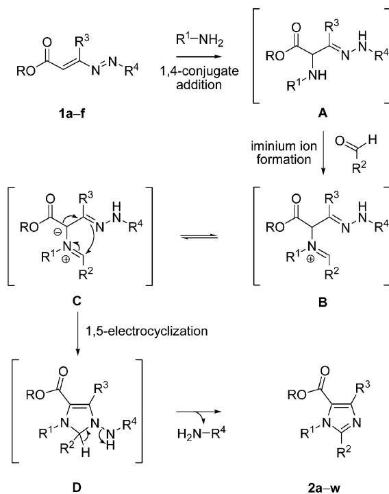
Scheme 1. Postulated mechanism for the formation of imidazole-4-carboxylates 2a–w from DDs 1a–f .
